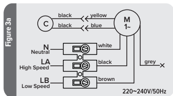
Wiring connection diagram for models with flange diameter 315 (for fans without speed switch button)
