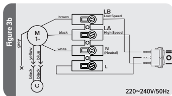
Wiring connection diagram for models with flange diameter 315 (for fans with speed switch button)
