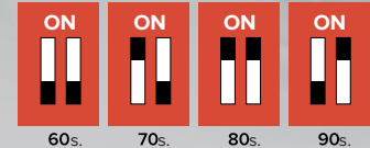
Switching delay
