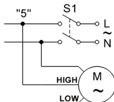
Wiring diagram for second speed
